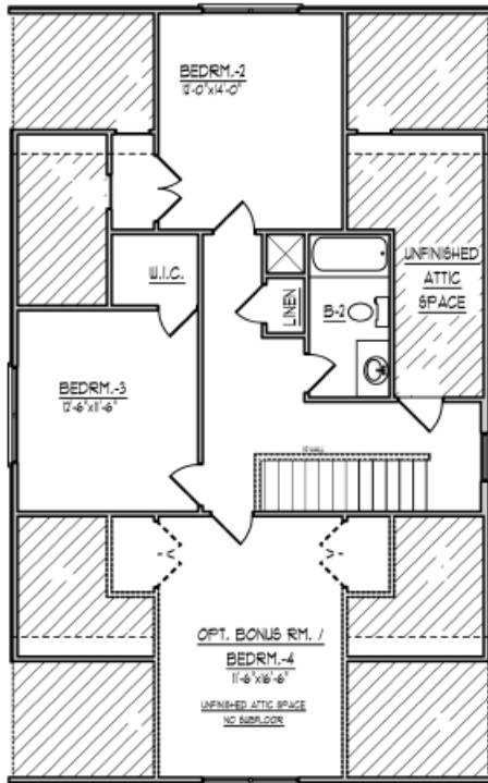
BASE PLAN
