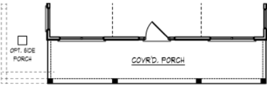
OPTIONAL 10'x16' SCREENED PORCH OPTIONAL 10'x12' SCREENED PORCH OPTIONAL SIDE PORCH FIRST FLOOR PLAN ELEVATION B
