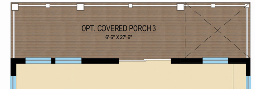
PARTIAL THIRD FLOOR PLAN W/ OPT. COVERED PORCH 3 OPT #00148
