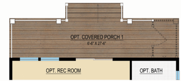
PARTIAL FIRST FLOOR PLAN W/ OPT. COVERED PORCH 1 OPT #00146
