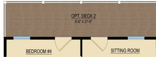
PARTIAL SECOND FLOOR PLAN W/ OPT. DECK 2 OPT #00156
