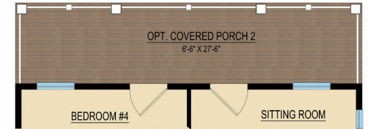
PARTIAL SECOND FLOOR PLAN W/ OPT. COVERED PORCH 2 OPT #00147
