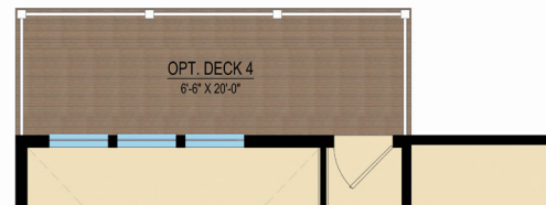
PARTIAL FOURTH FLOOR PLAN W/ OPT. DECK 4
