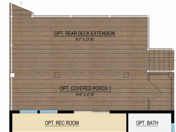
PARTIAL FIRST FLOOR PLAN W/ OPT. COVERED PORCH 1 AND OPT. REAR DECK EXTENSION
