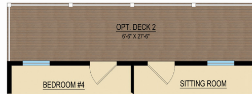
PARTIAL SECOND FLOOR PLAN W/ OPT. DECK 2
