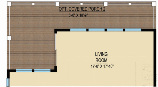
PARTIAL SECOND FLOOR PLAN W/ OPT. COVERED PORCH 2 OPT #00147
