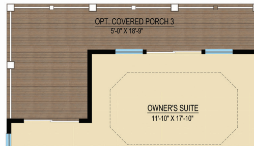
PARTIAL THIRD FLOOR PLAN OPTIONS SHOWN: SECOND SLIDING GLASS DOOR ILO CENTER WINDOWS W/ COVERED PORCH 3
