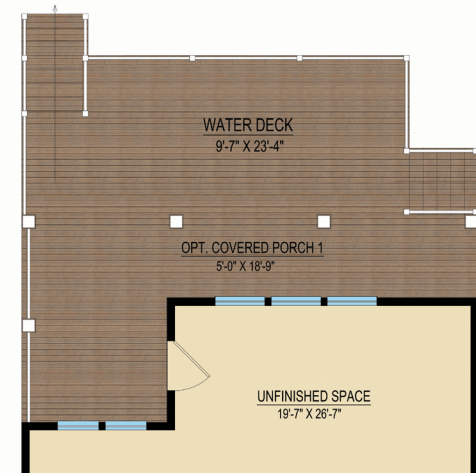
PARTIAL FIRST FLOOR PLAN W/ OPT. COVERED PORCH 1 AND OPT. WATER DECK OPT #00146 + OPT #00144
