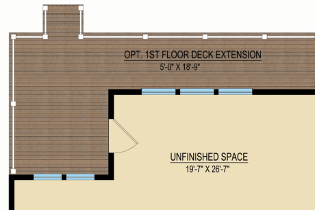
PARTIAL FIRST FLOOR PLAN W/ OPT. 1ST FLOOR DECK EXTENSION OPT #00143
