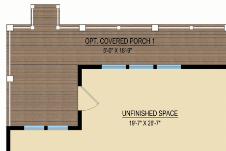
PARTIAL FIRST FLOOR PLAN W/ OPT. COVERED PORCH 1 OPT #00146
