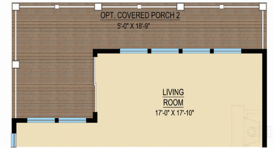
PARTIAL SECOND FLOOR PLAN W/ OPT. COVERED PORCH 2
