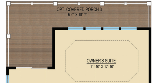
PARTIAL THIRD FLOOR PLAN W/ OPT. COVERED PORCH 3
