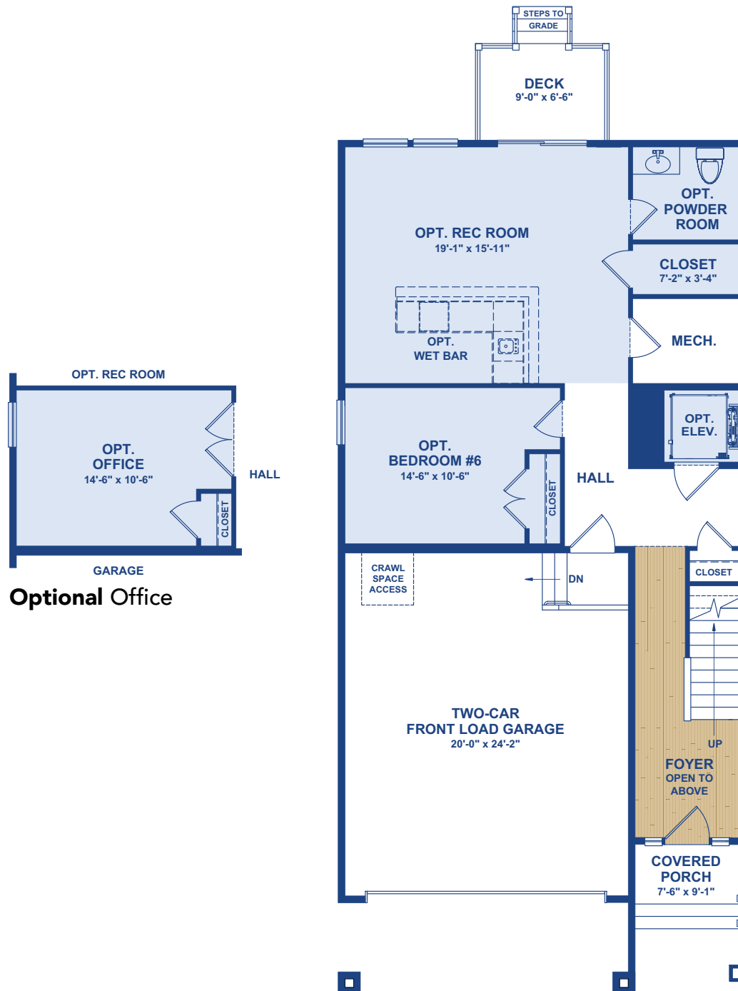
First Floor Plan With Popular Options
