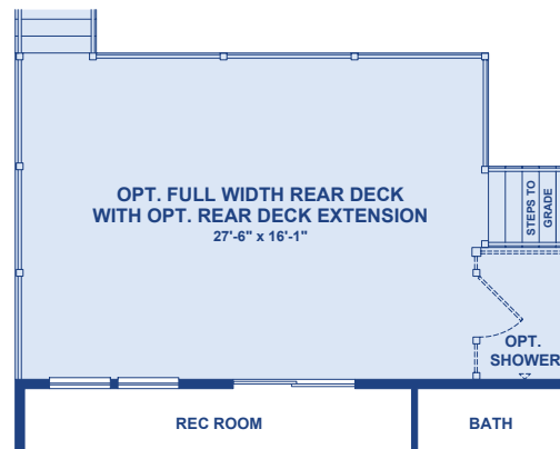
Optional Full Width Rear Deck with Optional Water Deck 00141 & 00144
