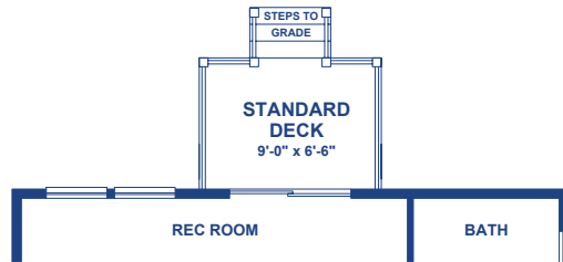
Standard Deck
