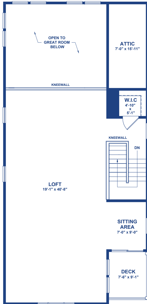
Standard Fourth Floor Plan
