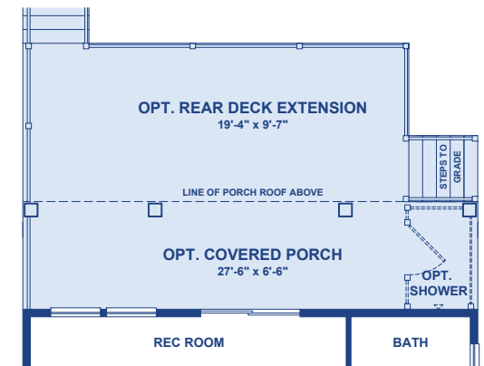
Optional Covered Porch 1 with Optional Water Deck 00146 & 00144
