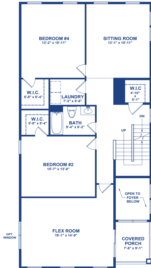
Standard Second Floor Plan
