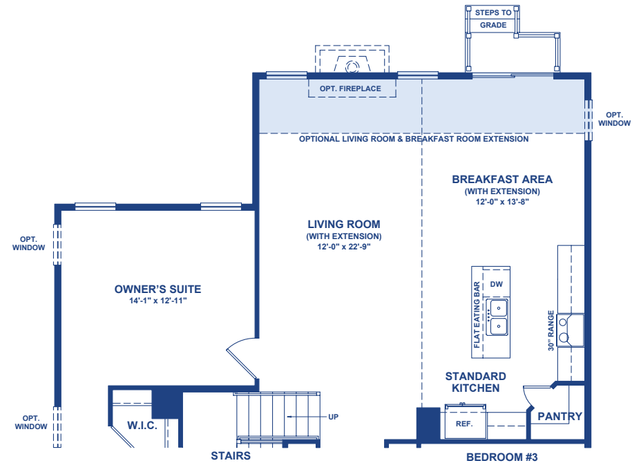
Optional Living Room / Breakfast Area Extension
