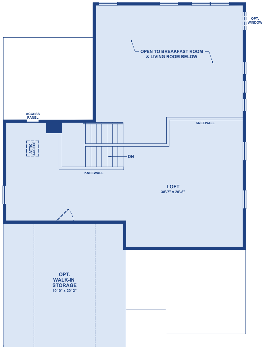
Optional Second Floor Loft Plan 00840
