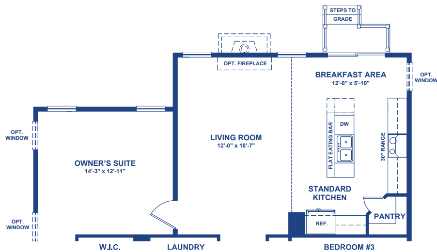
Standard First Floor Plan
