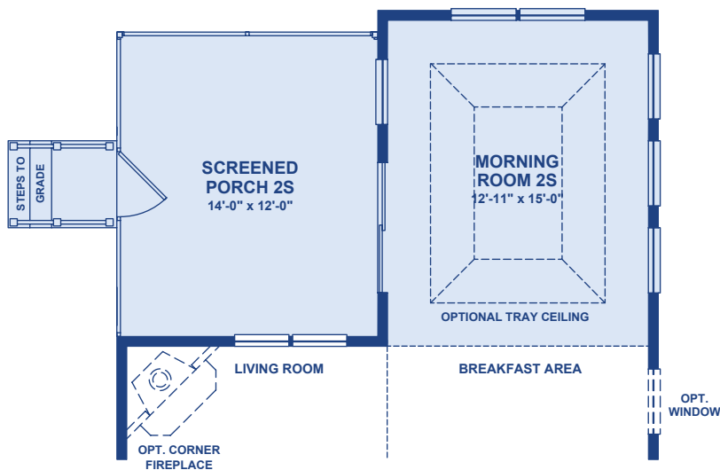
Optional Screened Porch 2S
