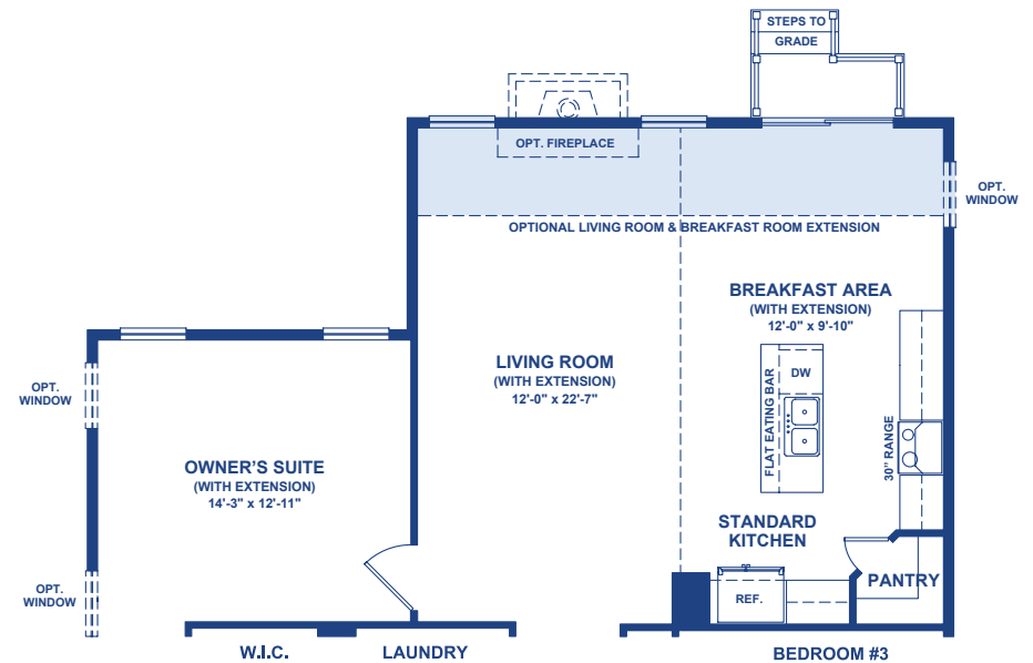
Optional Living Room / Breakfast Area Extension
