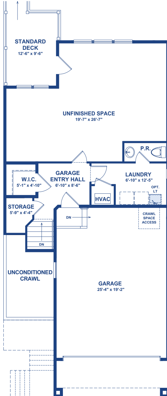
Standard First Floor Plan
