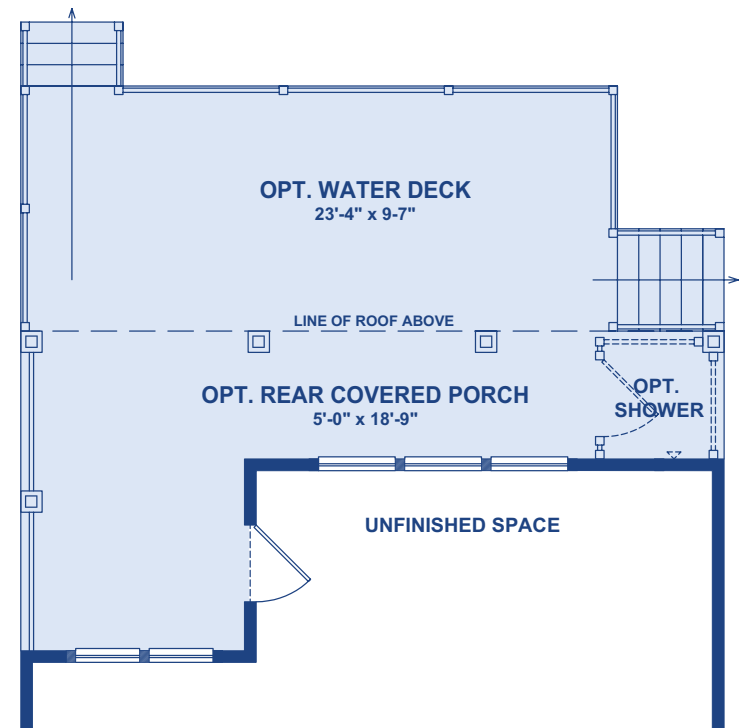
Optional Covered Porch 1 with Optional Water Deck 00144
