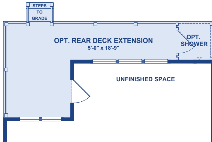
Optional First Floor Deck Extension 00143
