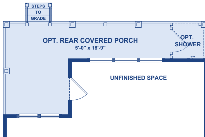
Optional First Floor Covered Porch 1 00146
