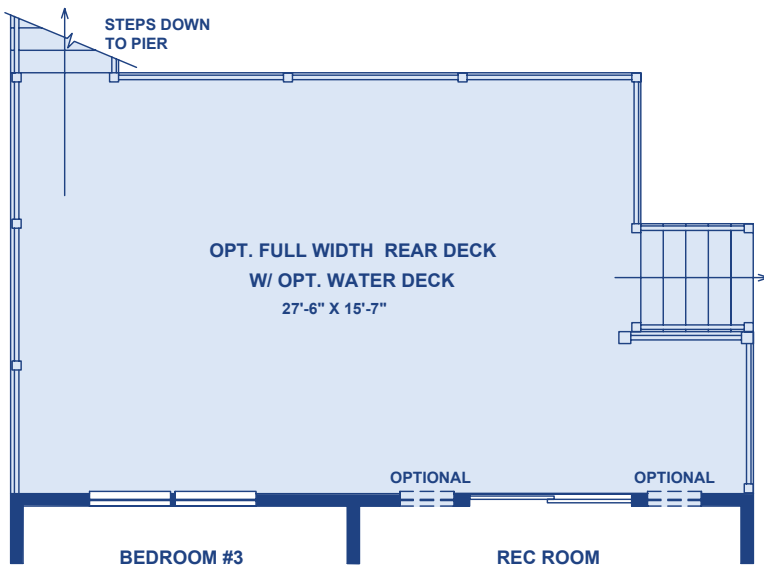
Optional First Floor Full Width Rear Deck with Water Deck 00144
