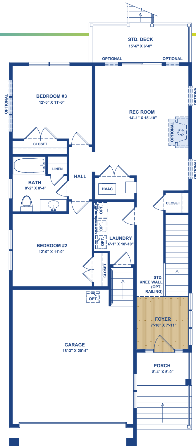
Standard First Floor Plan (Cottage Elevation Shown)
