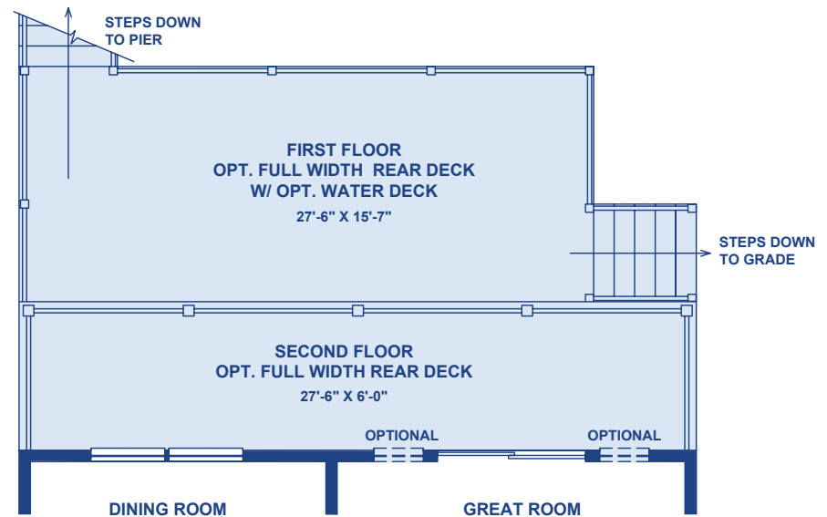
Optional Second Floor Full Width Rear Deck 00156 (includes First Floor Full Width with Water Decks below) 00137
