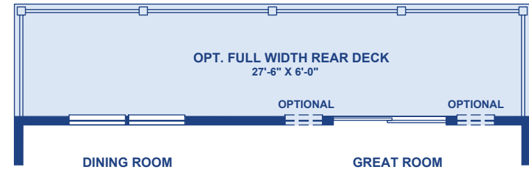
Optional Second Floor Full Width Rear Deck (includes First Floor Full Width Rear Deck below) 00156
