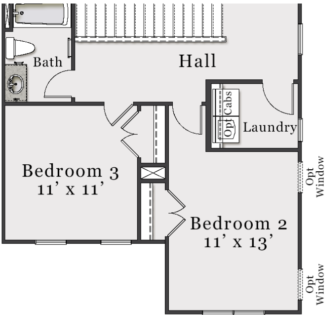
B Second Floor
