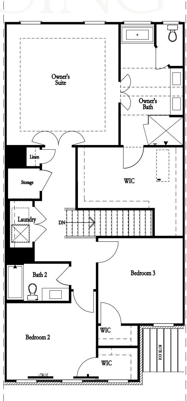
SECOND FLOOR
