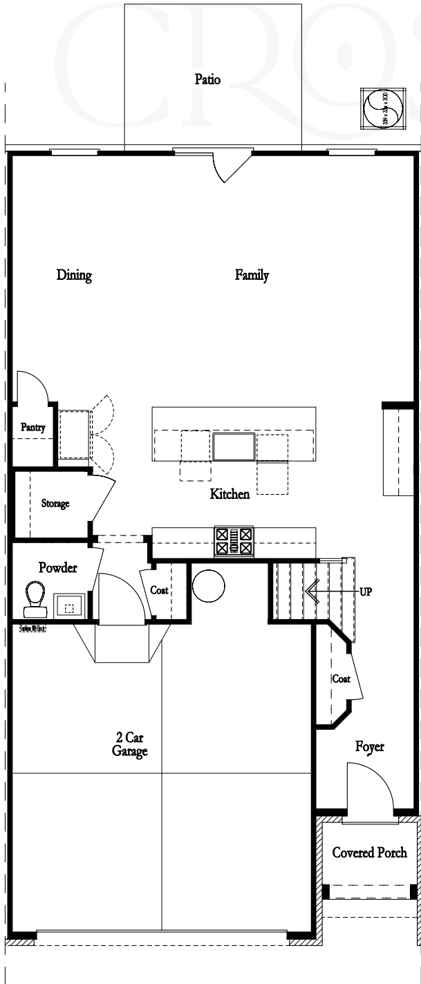
FIRST FLOOR
