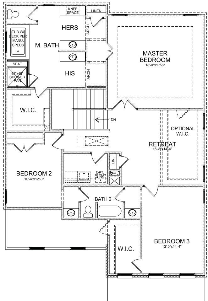
SECOND FLOOR
