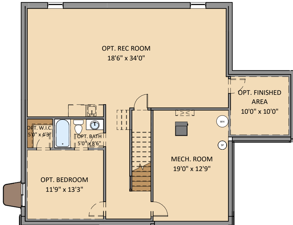
Finished Basement Plan with Buried Condition
