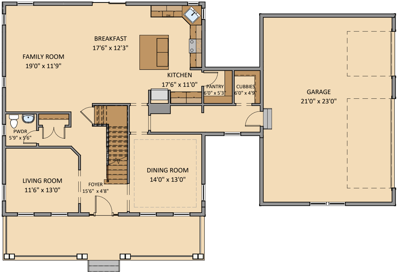
First Floor Plan - Elevation 2 with 3-Car Garage
