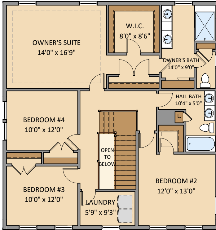
2nd Floor Plan - Elevation 1
