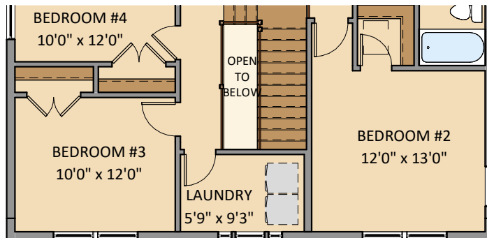
2nd Floor Plan - Elevation 2
