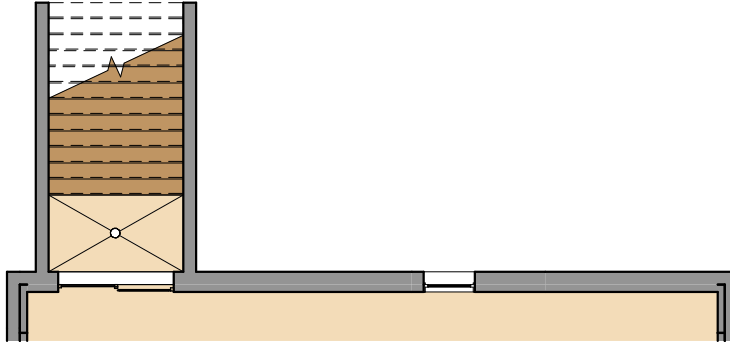
Finished Basement Plan with Areaway Condition
