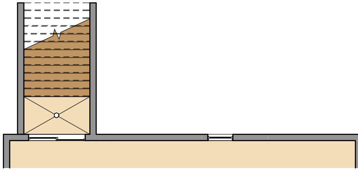
Unfinished Basement Plan with Areaway Condition
