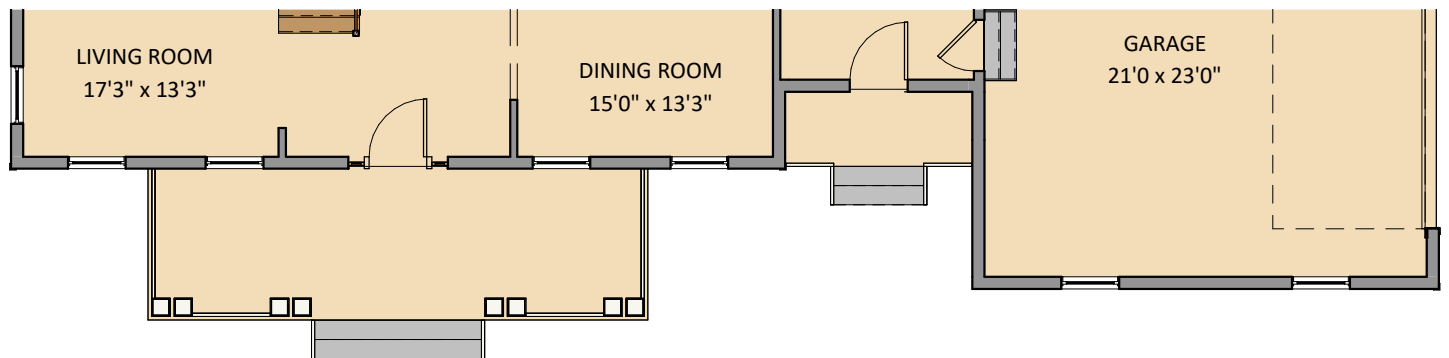
First Floor Plan - Elevation 2 with 2nd Entry
