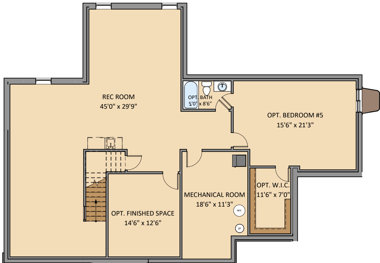
Finished Basement Plan with Buried Condition
