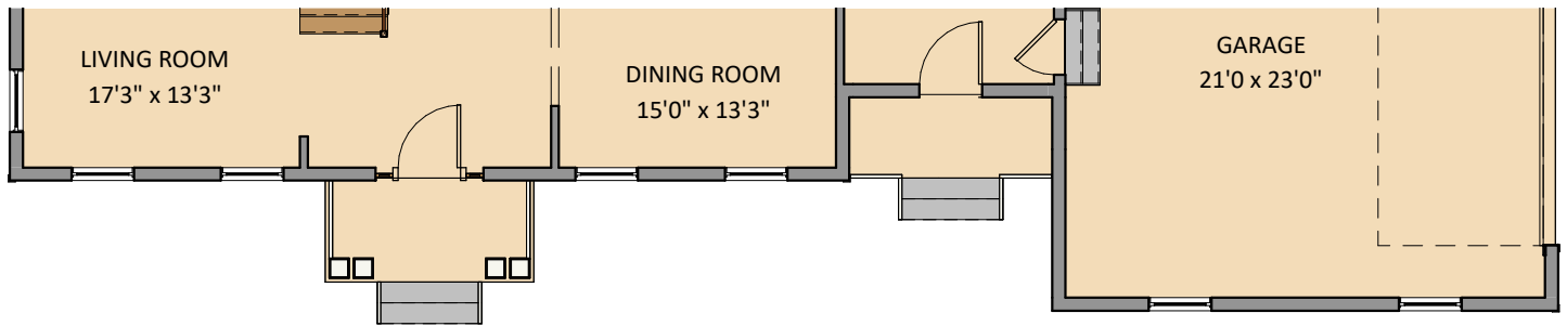
First Floor Plan - Elevation 1 with 2nd Entry
